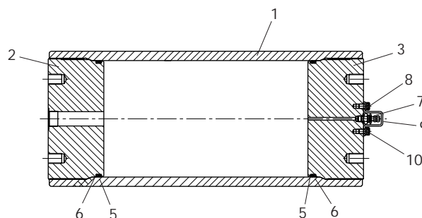
180mm and 250mm Bore Gas Bottles
