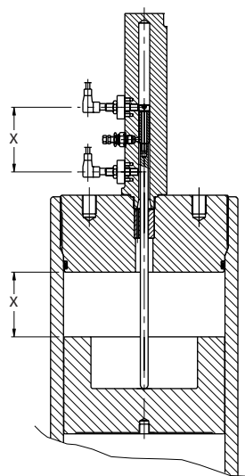
Standard Cored-Type Gas Valve
